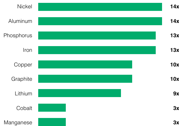
2019 vs 2030 demand growth
